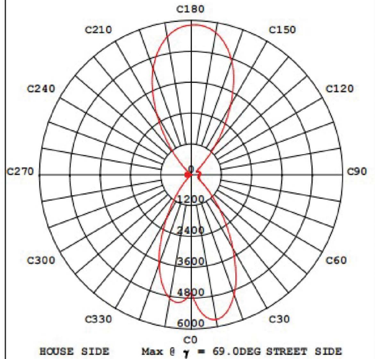
MAX INTENSITY CONE SURFACE DISTRIBUTION DIAGRAM
