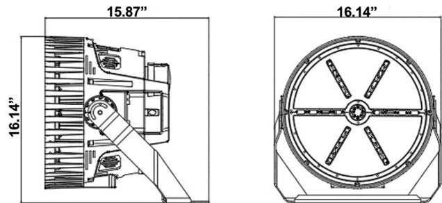
Standard Yoke mount
