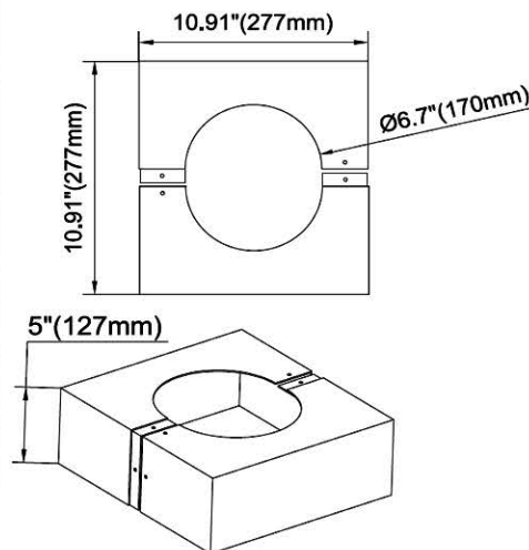
6.5" Flange Base Cover Size
