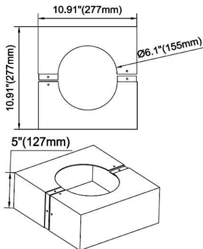
6" Flange Base Cover Size
