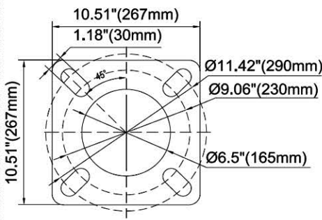
6.5" Flange
