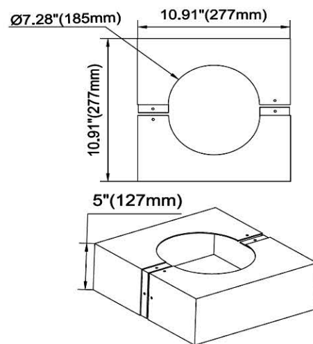
7" Flange Base Cover Size
