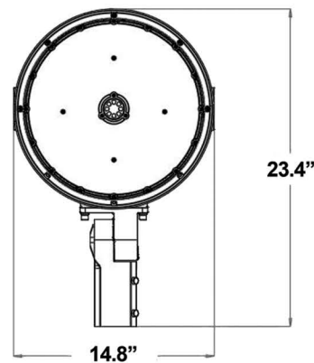
Slip Fitter Mount
