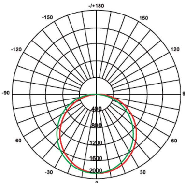
2PT-20/30/40/60W-3CCT-PC 60W @ 5000K
