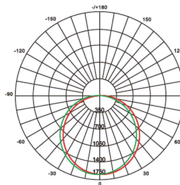
2PT-20/30/40/60W-3CCT-PC 30W @ 5000K
