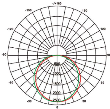
2PT-80/100/120/150W-3CCT-PC 120W @ 5000K
