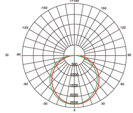
2PT-80/100/120/150W-3CCT-PC 100W @ 5000K
