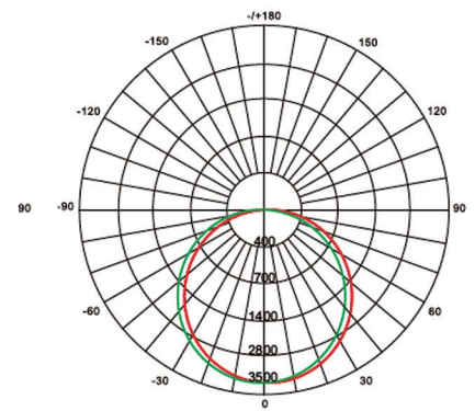
2PT-20/30/40/60W-3CCT-PC 40W @ 5000K
