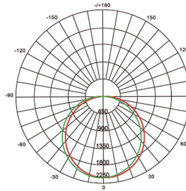
2PT-80/100/120/150W-3CCT-PC 80W @ 5000K
