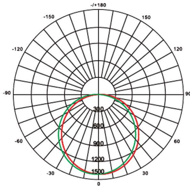
2PT-20/30/40/60W-3CCT-PC 20W @ 5000K
