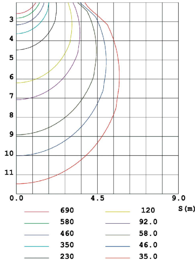
C0 PLANE ISOLUX DIAGRAM (UNIT:lx) MH (m)
