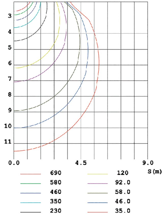
CO PLANE ISOLUX DIAGRAM (UNIT:lx)
