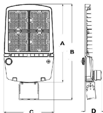
Trunnion mount
